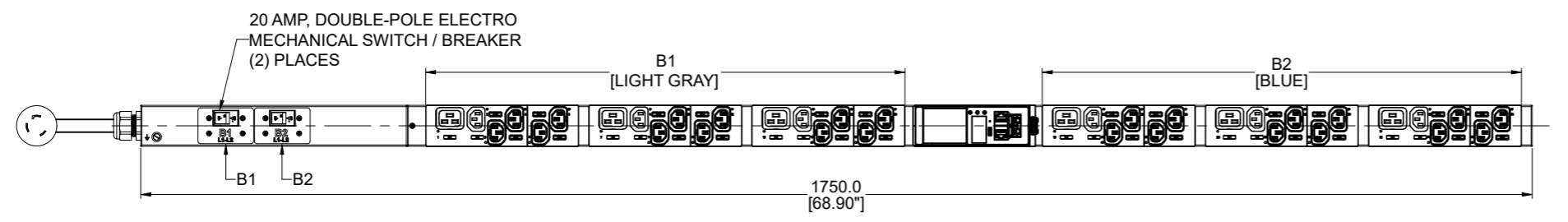
FRONT VIEW
