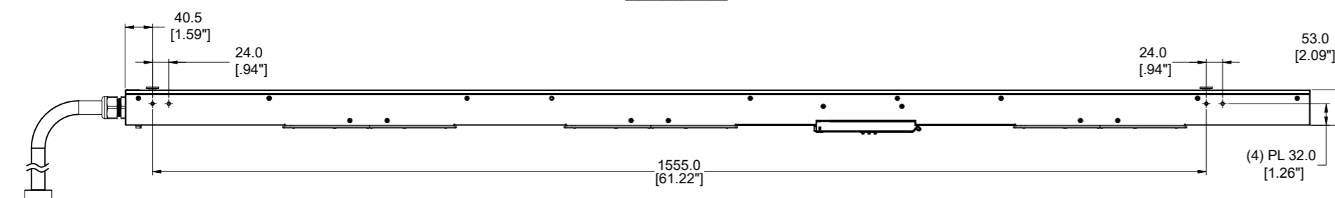
BOTTOM VIEW
