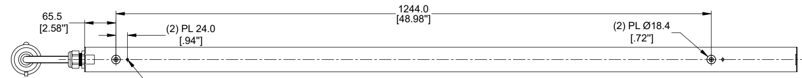
REAR VIEW
