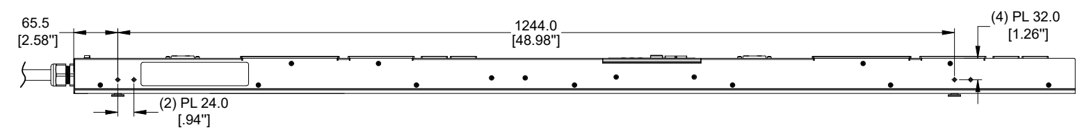
LEFT VIEW
