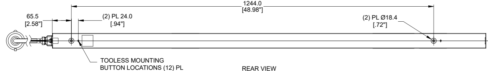
REAR VIEW
