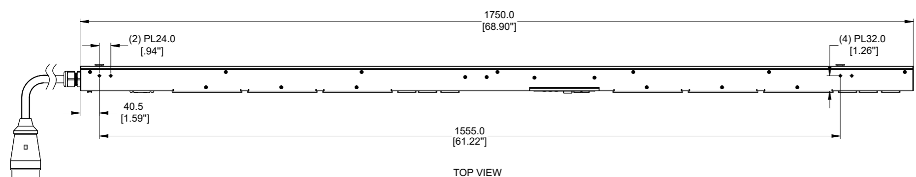
REAR VIEW
