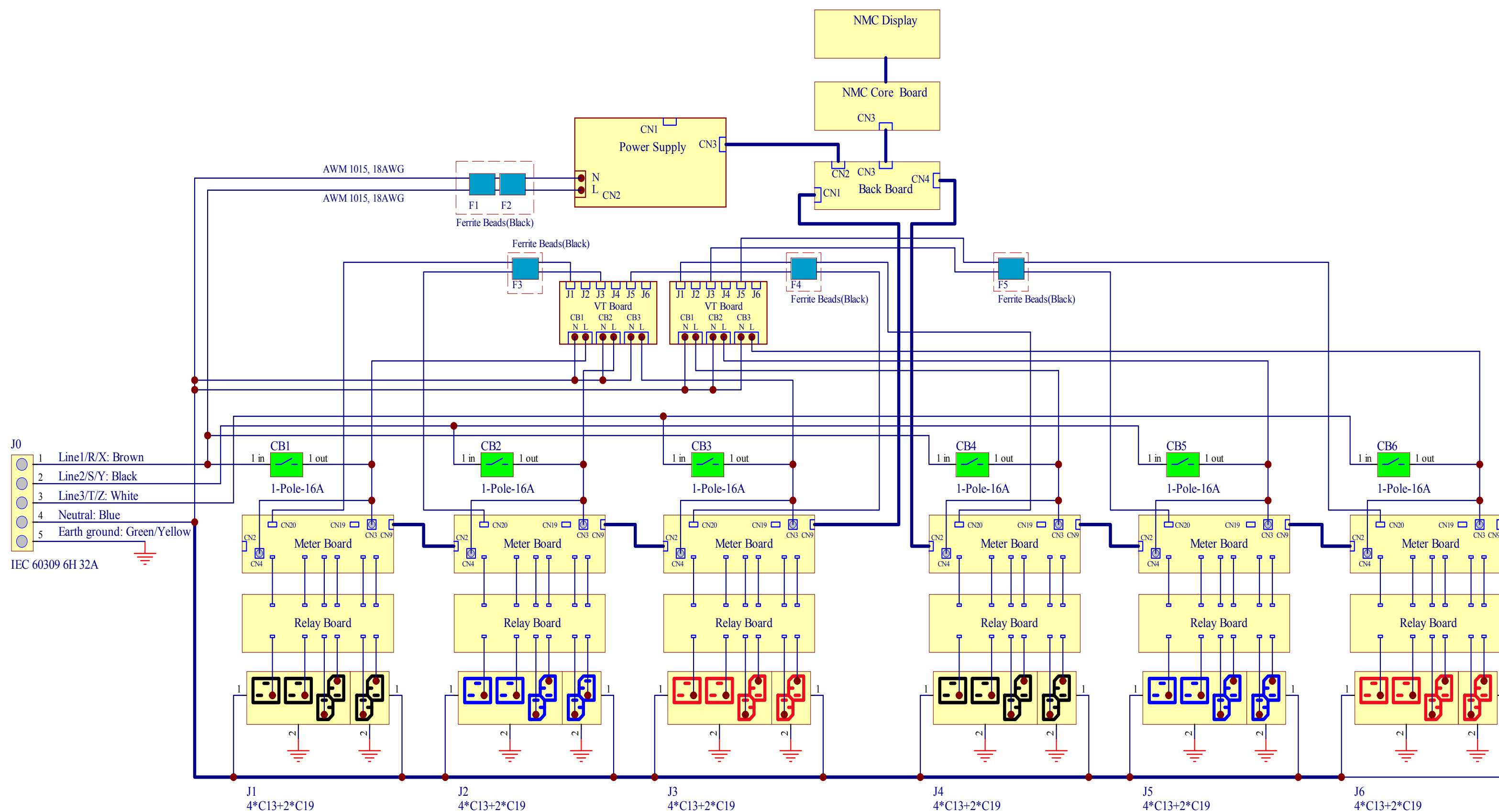
INTERNAL WIRING SCHEMETIC
